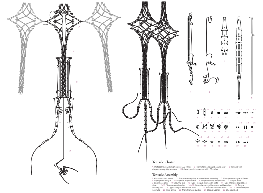
Figure 2. Flexible meshwork systems arranged in clusters support mounted kinetic tentacles activated by optic sensors.
